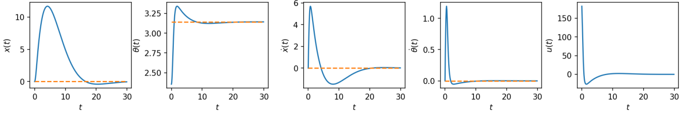
Figure 2: Infinite-horizon LQR controller for cart-pole balance
