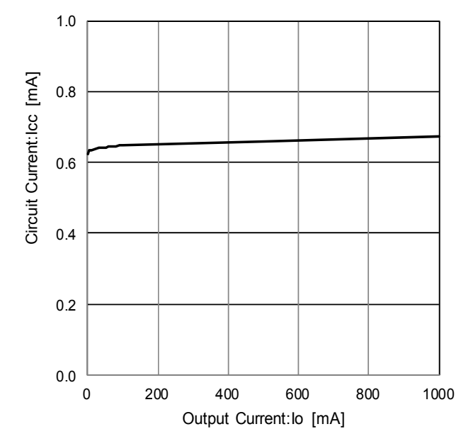
Figure 67. Circuit Current
