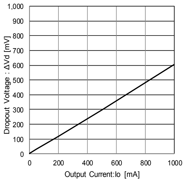
Figure 52. Dropout Voltage ( V_{cc}=V_o \times 0.95V )
