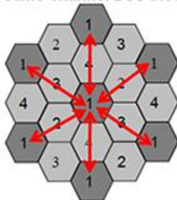
Increased Frequency Reuse (w/ 80 MHz channels) - All same-channel BSS blocking
