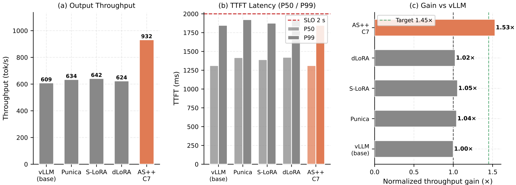
Figure 2: AS++ vs SOTA — K=10, r=32, \lambda=7 req/s, A6000 TP=1 (E13.11)
