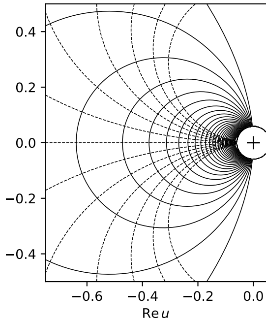
(b) \text{Re } \Phi_{\text{att}} \in \mathbb{Z} (solid), \text{Im } \Phi_{\text{att}} \in \frac{1}{2}\mathbb{Z} (dashed)
