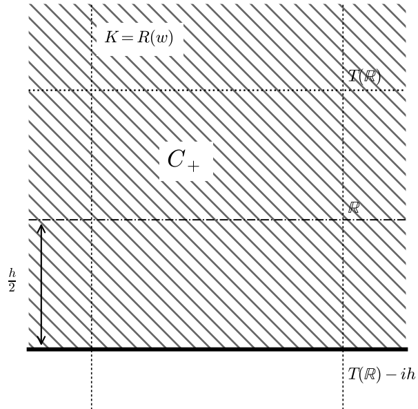
(b) attracting time w
