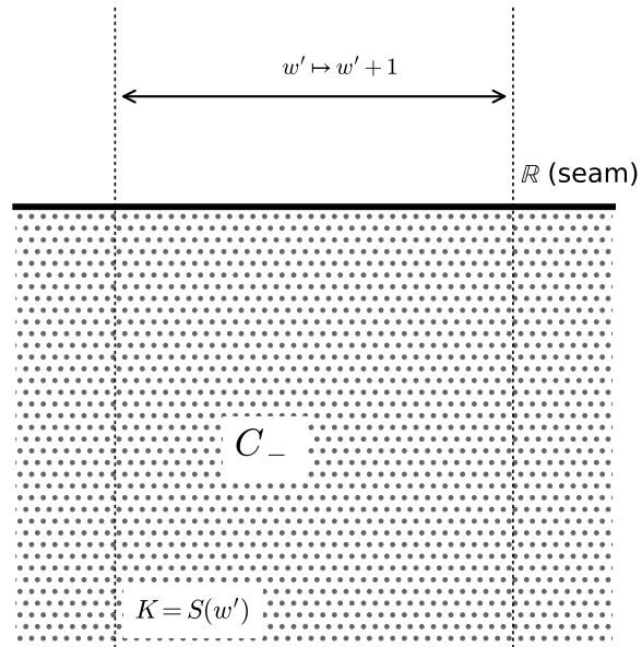
(a) repelling time w'
