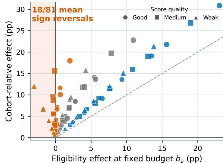
(a) Joint and fixed-budget effects
