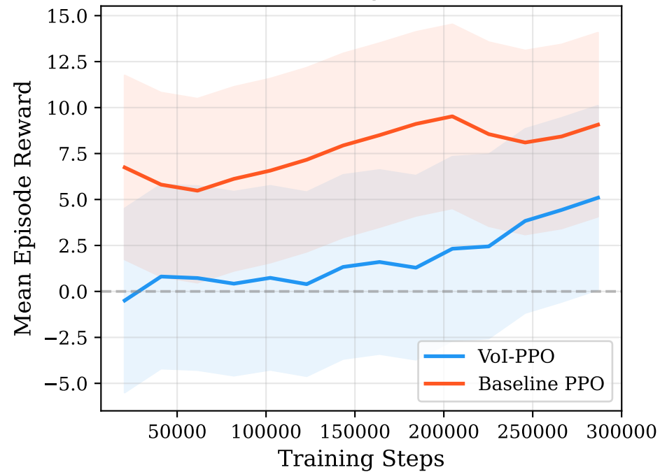
(a) Training Reward
