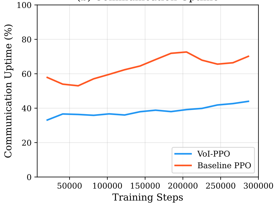
(b) Communication Uptime
