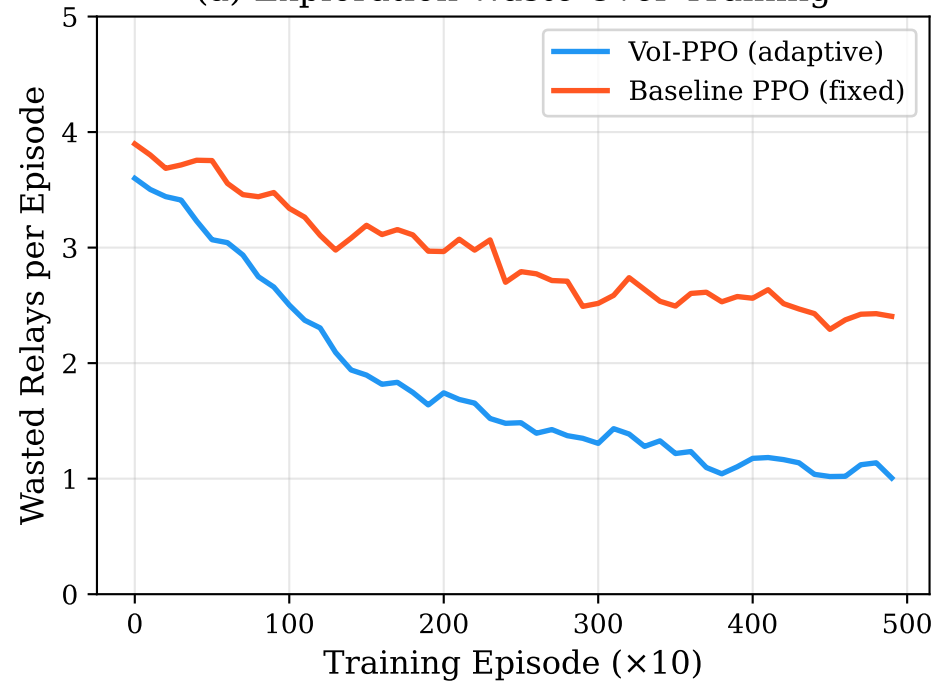
(a) Exploration Waste Over Training
