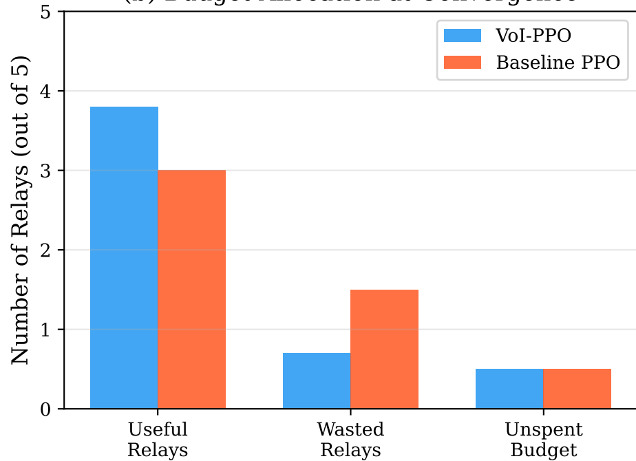
(b) Budget Allocation at Convergence
