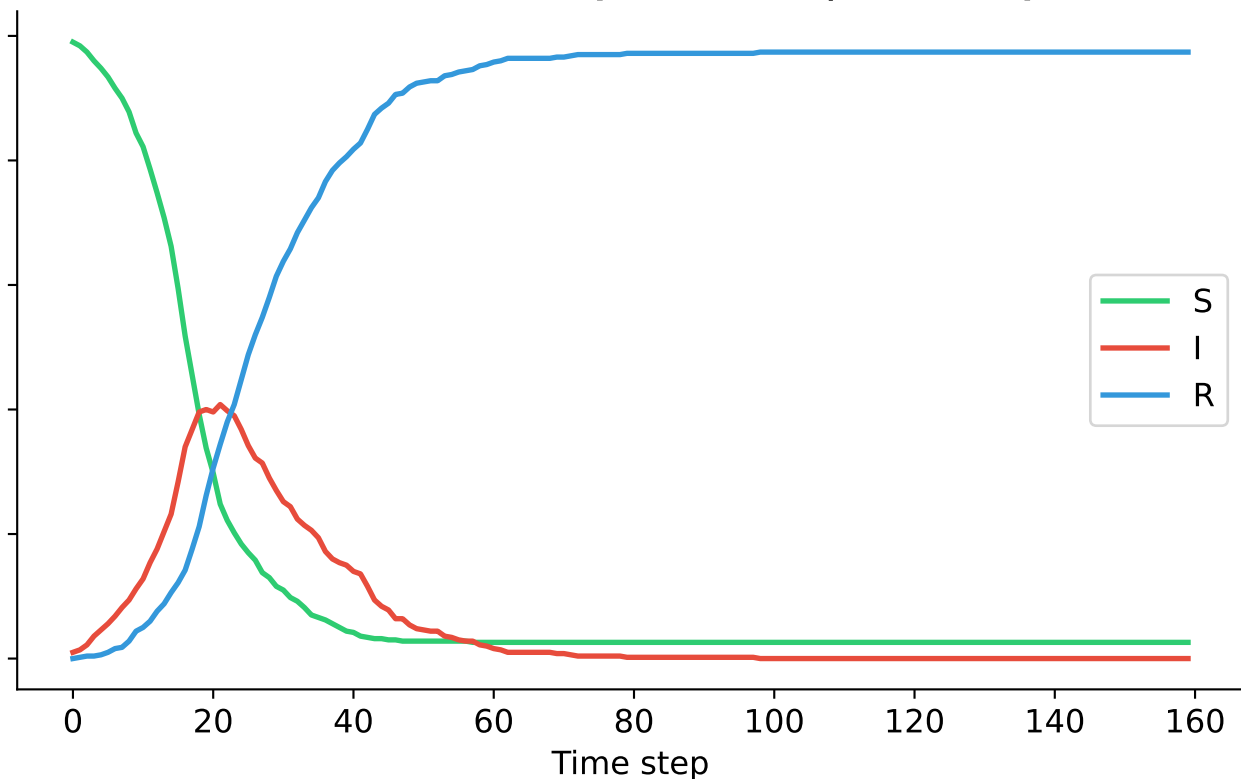
Well-mixed ABM (stochastic, one run)
