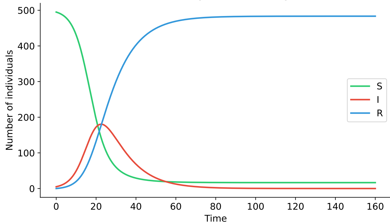
ODE SIR (deterministic)
