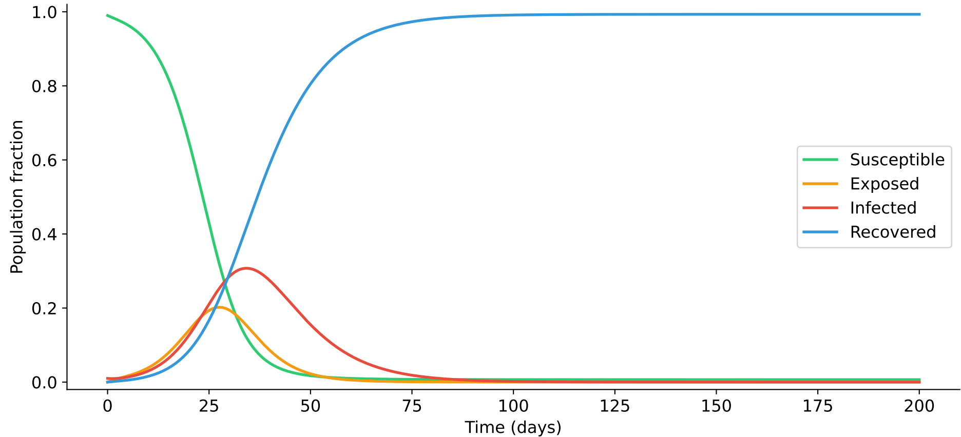
SEIR Model Dynamics ( R_0 = 5 , latent period = 5 days)
