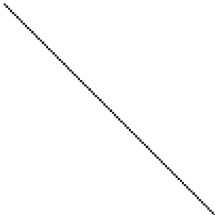
Rule 184
