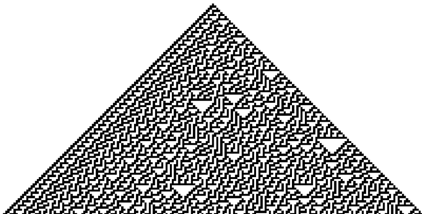
Rule 30
