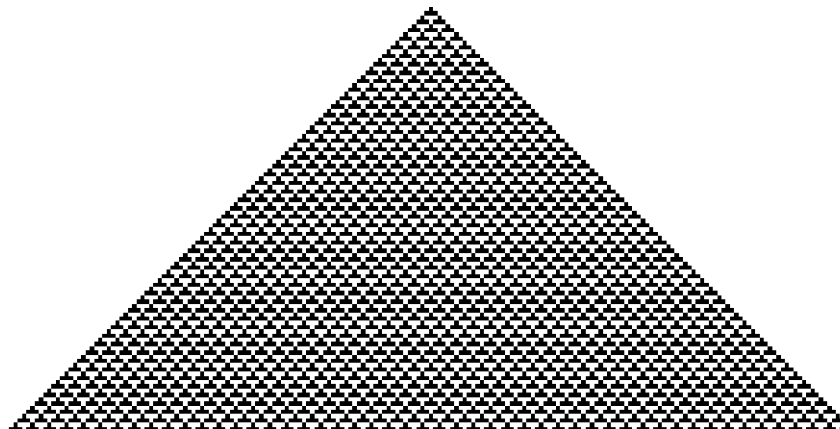
Rule 54
