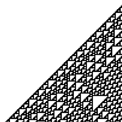
Rule 110
