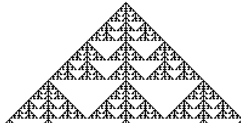
Rule 150
