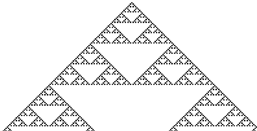
Rule 90
