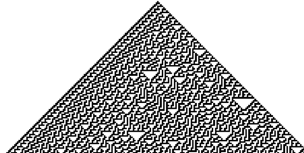
Class III — Rule 30
