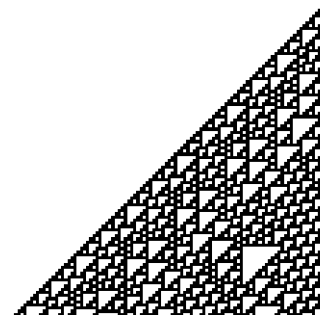
Class IV — Rule 110
