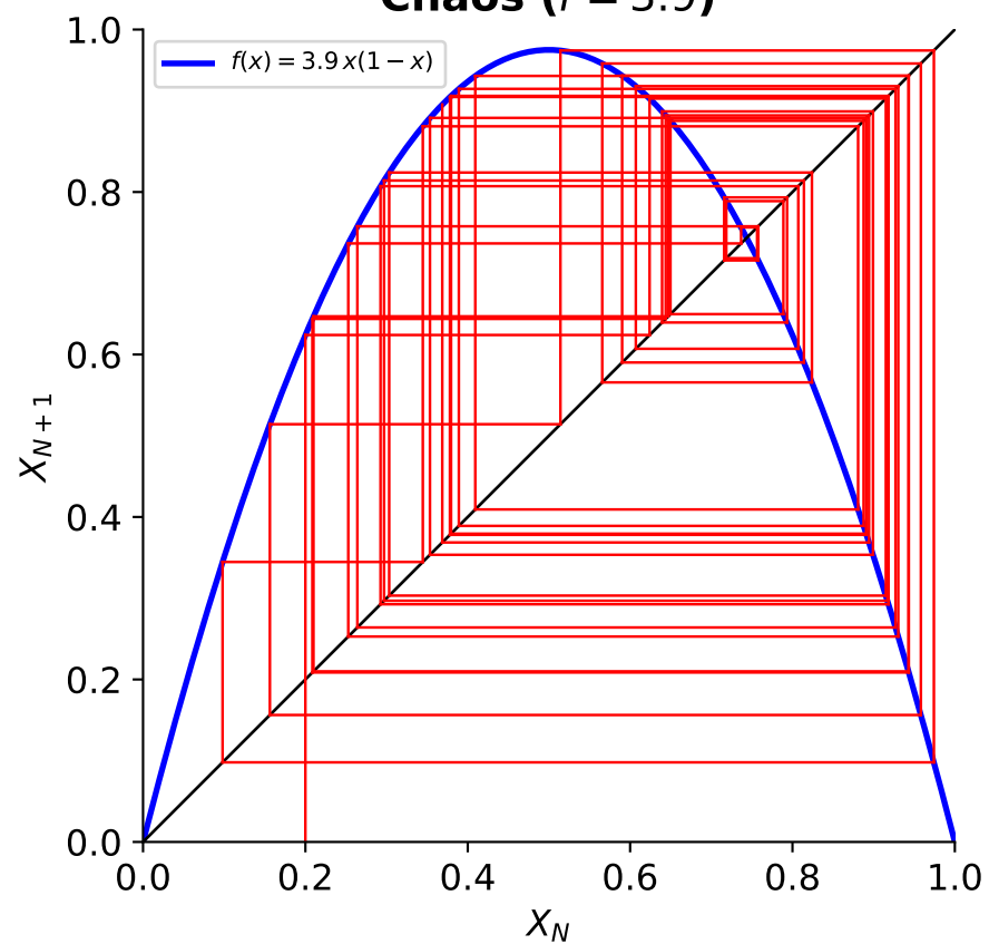
Chaos ( r = 3.9 )
