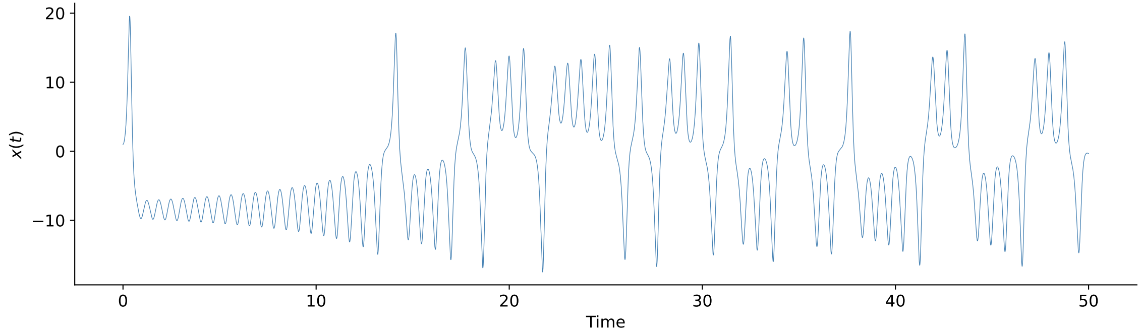
Lorenz System — x component over time
