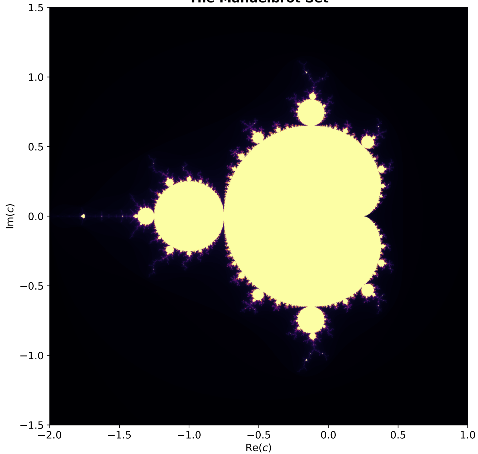
The Mandelbrot Set
