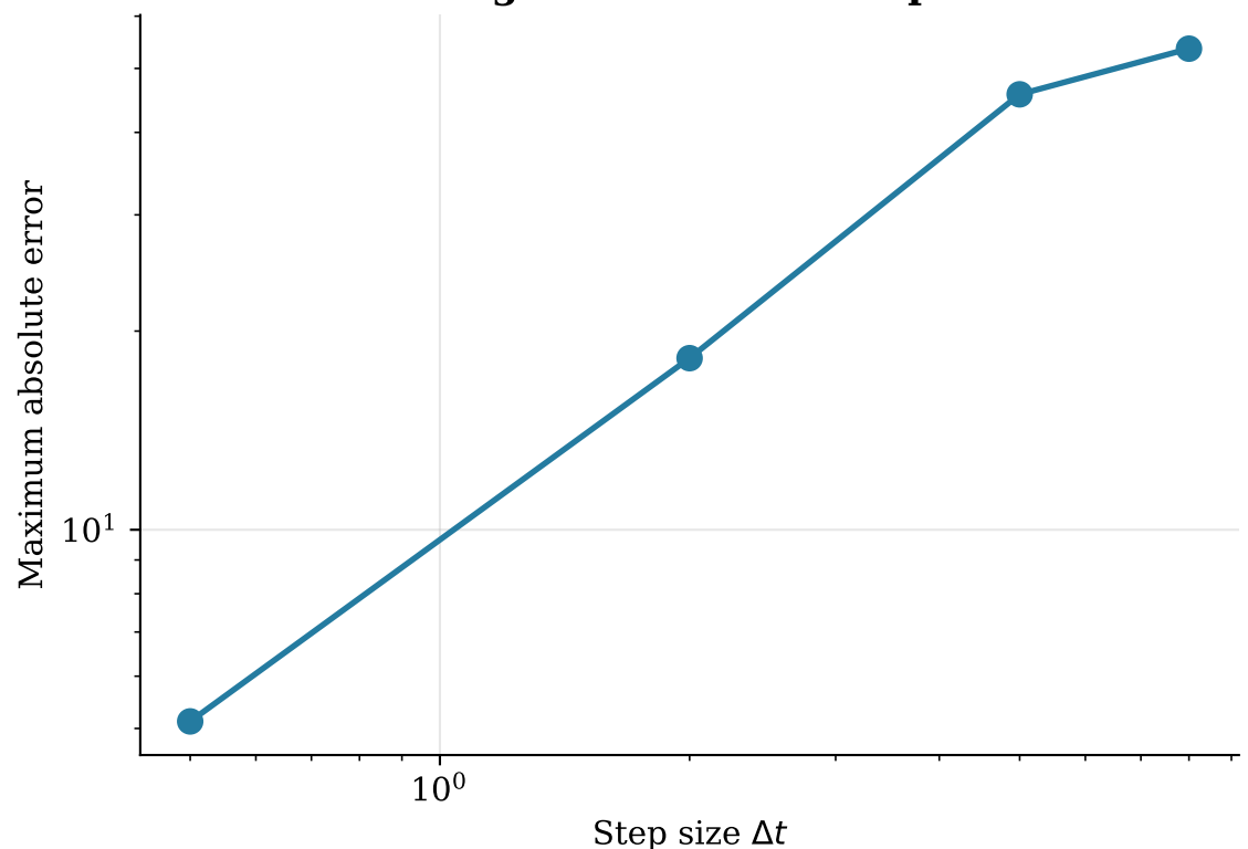
Convergence: Error vs Step Size
