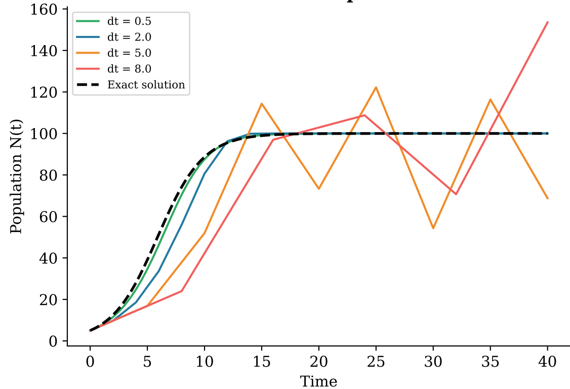
Euler Method: Step Size Effect
