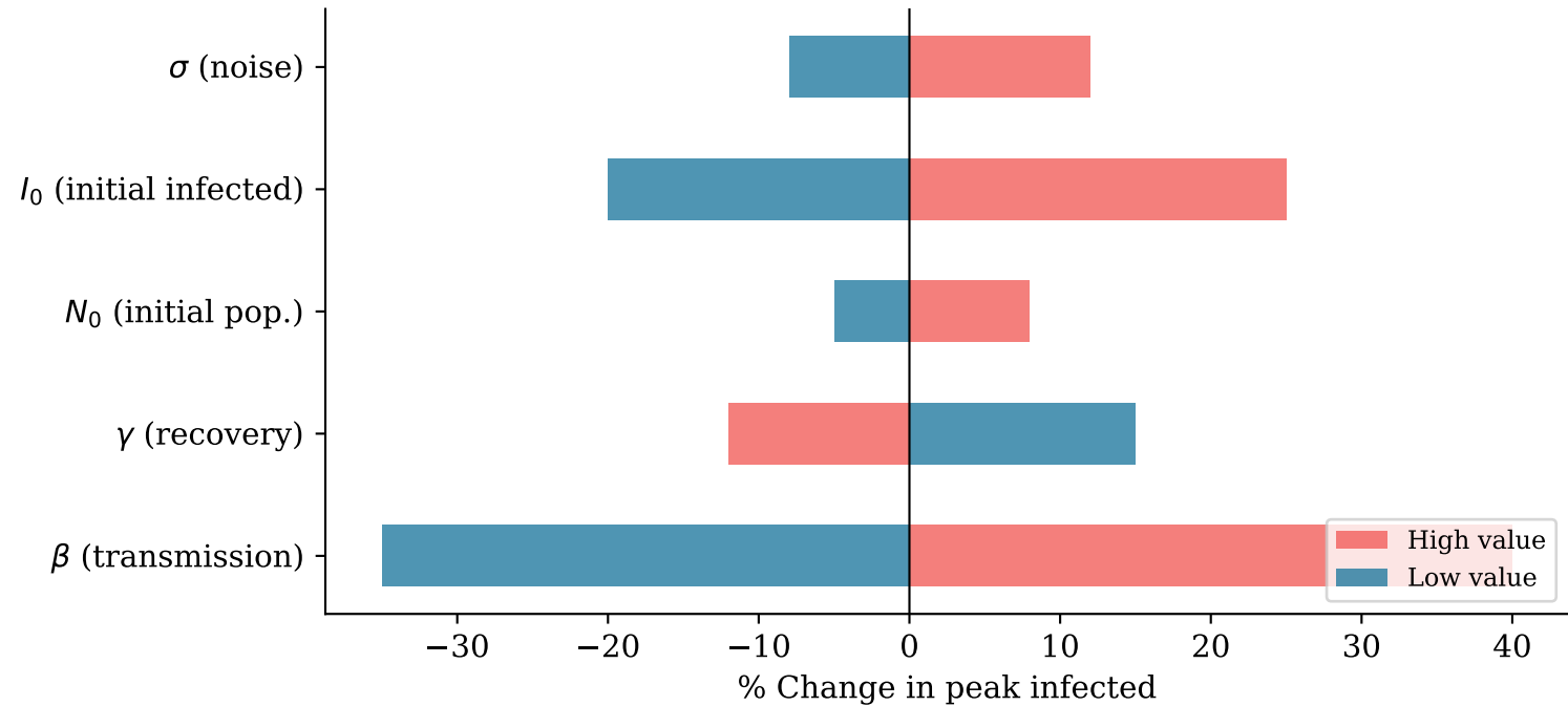
Tornado Diagram: Parameter Sensitivity of SIR Peak
