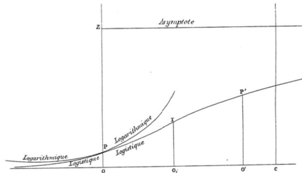
Verhulst and the first plot of the logistic growth curve
