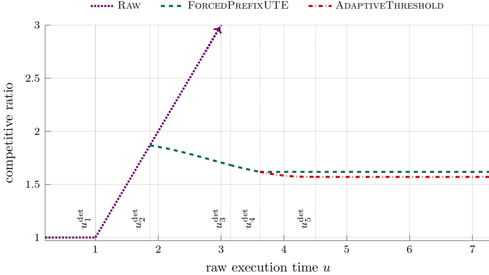
Figure 1: The guarantees of the three deterministic policies. The arrow on RAW marks its off-scale linear continuation; the teal horizontal line is the \varphi guarantee of zero-prefix FORCEDPREFIXUTE.
