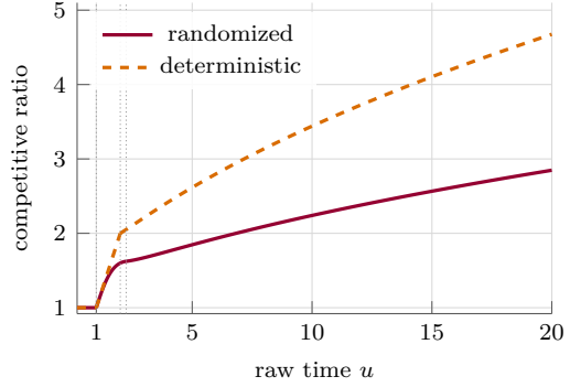
Figure 1: The exact deterministic and randomized ratios for blind optimization.
