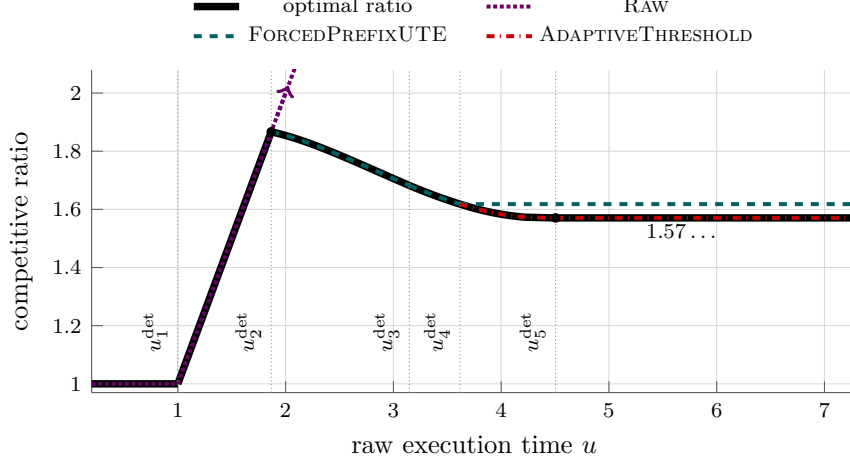
Figure 2: The guarantees of the three deterministic policies and their exact lower envelope. The black outline is the optimal ratio. The arrow on RAW marks its off-scale linear continuation; the teal horizontal line is the \varphi guarantee of zero-prefix FORCEDPREFIXUTE.
