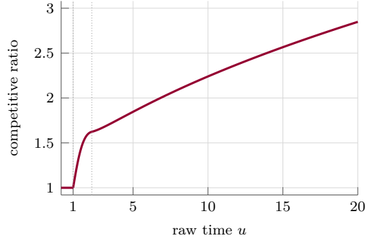
Figure 1: The exact randomized ratio for blind optimization.
