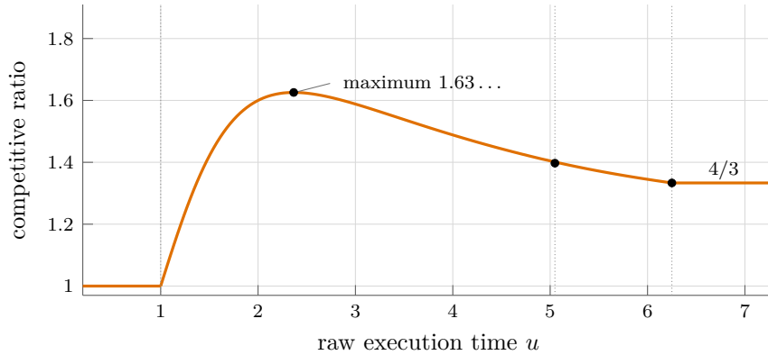
Figure 3: The exact randomized revealing-optimization ratio as a function of the raw execution time u .
