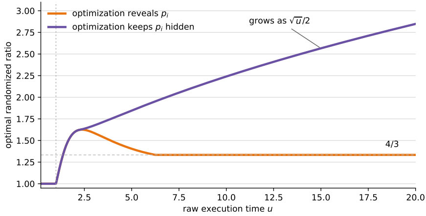
Figure 4: Revealing p_i keeps the randomized revealing-optimization ratio bounded and eventually gives the 4/3 plateau. If optimization changes the processing time but does not reveal it before execution, the exact ratio instead grows as \sqrt{u}/2 .
