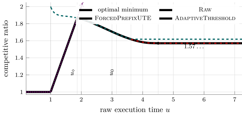
Figure 2: The three deterministic policy guarantees as functions of the raw execution time u . Their pointwise minimum, shown with a black outline, is the exact deterministic ratio. The arrow on RAW marks its off-scale linear continuation.
