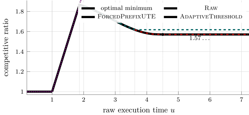
Figure 2: The three deterministic policy guarantees as functions of the raw execution time u . Their pointwise minimum, shown with a black outline, is the exact deterministic ratio.
