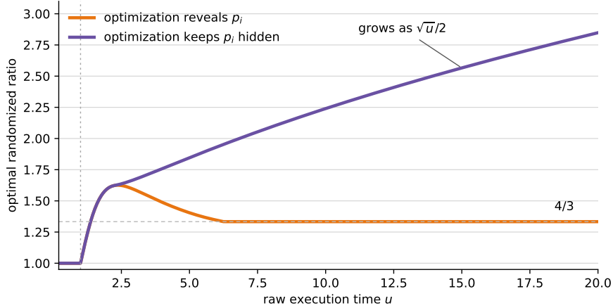
Figure 2: Revealing p_i keeps the randomized common-upper ratio bounded and eventually gives the 4/3 plateau. If optimization changes the processing time but does not reveal it before execution, the exact ratio instead grows as \sqrt{u}/2 .
