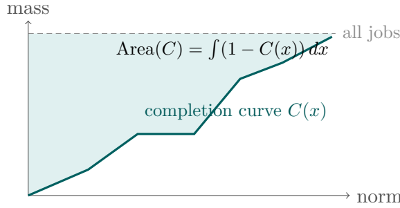
Figure 3: A fluid completion curve. Total completion cost is the shaded area between completed mass and total mass.
