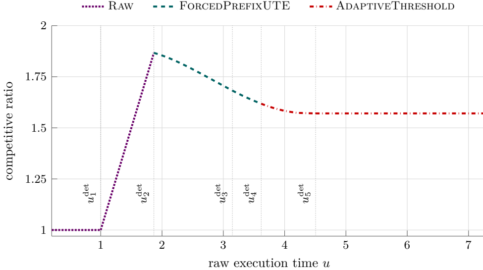
Figure 2: The three deterministic algorithms, each shown only on the range where it gives the best guarantee.
