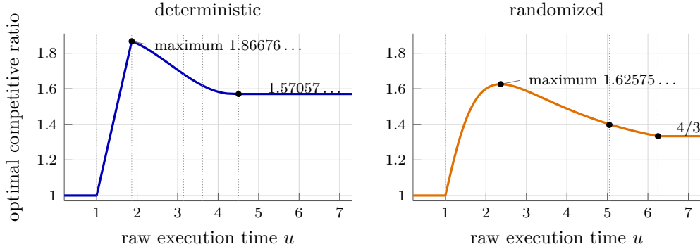
Figure 1: The exact asymptotic ratios as a function of the raw execution time u . Testing is pointless on the left. On the right, both curves reach their obligatory-testing values.
