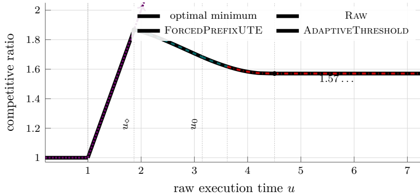
Figure 2: The three deterministic policy guarantees as functions of the raw execution time u , each shown on the range proved in the paper. Their pointwise minimum, shown with a black outline, is the exact deterministic ratio. The arrow on RAW marks its off-scale linear continuation.
