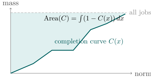
Figure 2: A fluid completion curve. Total completion cost is the shaded area between completed mass and total mass.
