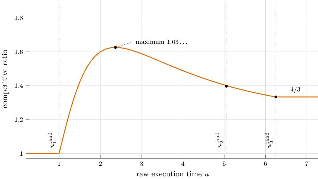
Figure 3: The exact randomized revealing-optimization curve. The two binary hard-instance families switch at the marked transition points.
