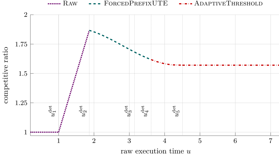
Figure 1: The three deterministic algorithms, each shown only on the range where it gives the best guarantee.
