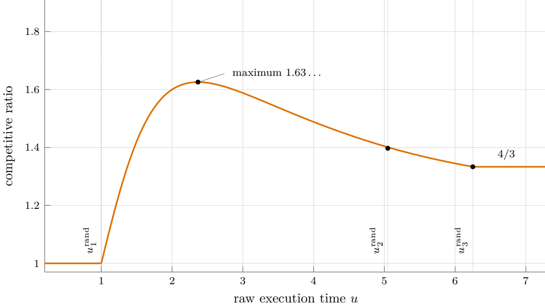
Figure 3: The exact randomized revealing-optimization curve. The two binary hard-instance families switch at the marked transition points.
