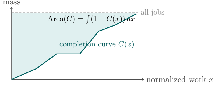
Figure 2: A fluid completion curve. Total completion cost is the shaded area between completed mass and total mass.
