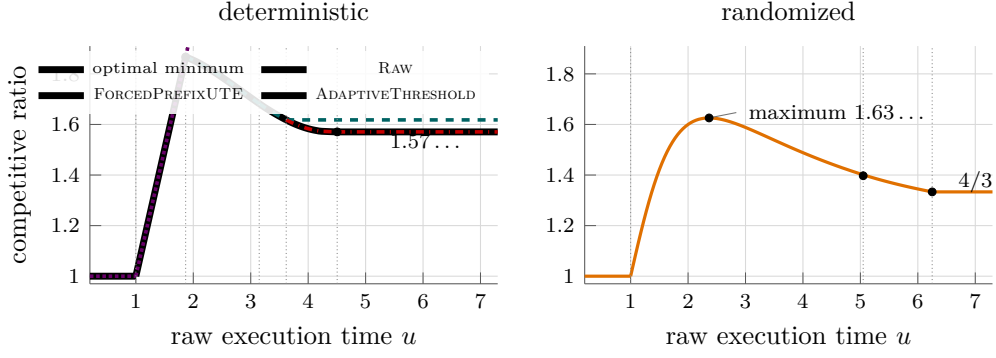
Figure 2: The exact asymptotic ratios as a function of the raw execution time u . In the deterministic panel, the three styled curves are the guarantees of RAW, FORCEDPREFIXUTE, and ADAPTIVETHRESHOLD; the black-outlined curve is their pointwise minimum. Testing is pointless on the left. On the right, both optimal curves reach their obligatory-testing values.
