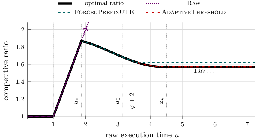
Figure 2: The three proved deterministic policy guarantees and their exact lower envelope. The black outline is the optimal ratio. The arrow on RAW marks its off-scale linear continuation; the teal horizontal line is the \varphi guarantee of zero-prefix FORCEDPREFIXUTE.
