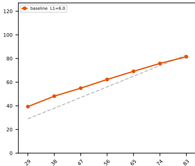
Audio Flamingo
