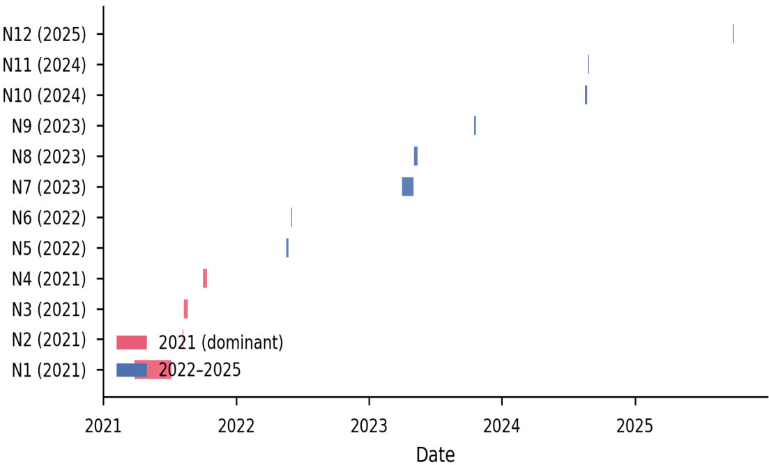
Fig. 2 — Temporal distribution of the 12 N-defined bloom events
