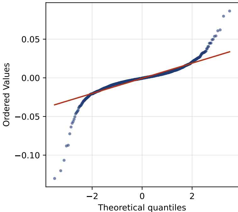
Normal QQ-plot: tails bend off the line
