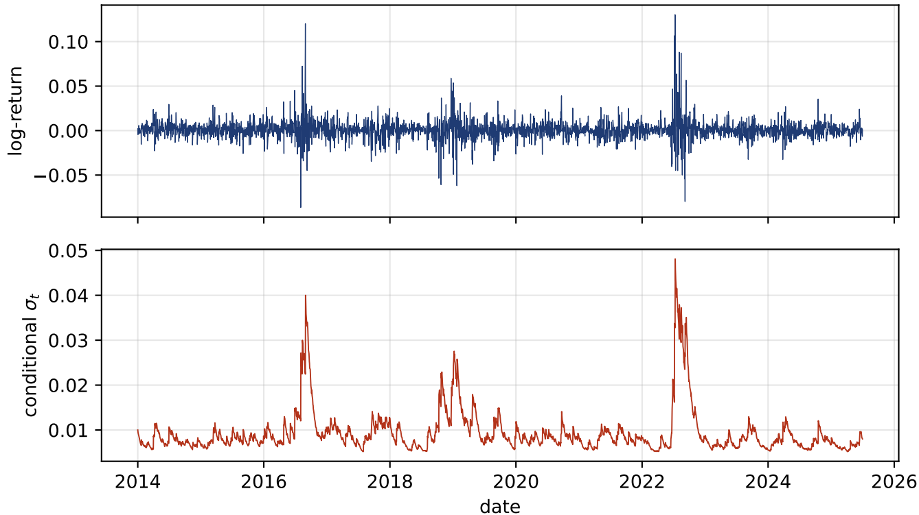
Daily returns: calm and storm cluster in time
