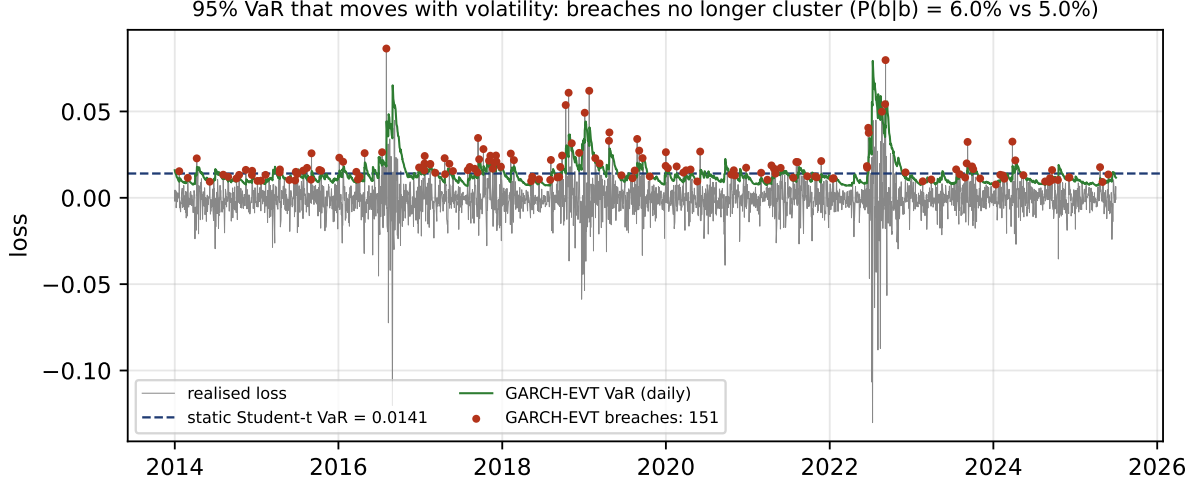
Figure 6: GARCH-EVT 95% VaR (green) rises into the 2016 and 2022 storms and relaxes after them. Its breaches are spread across the sample instead of bunched into the volatile spells.
