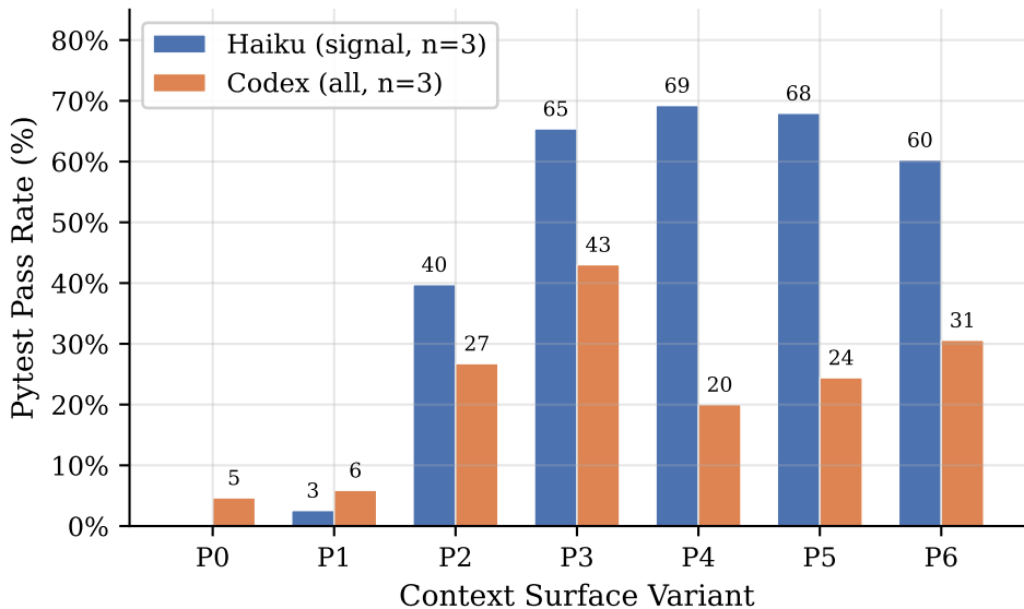
Surface Hierarchy: Pytest Pass Rates by Variant
