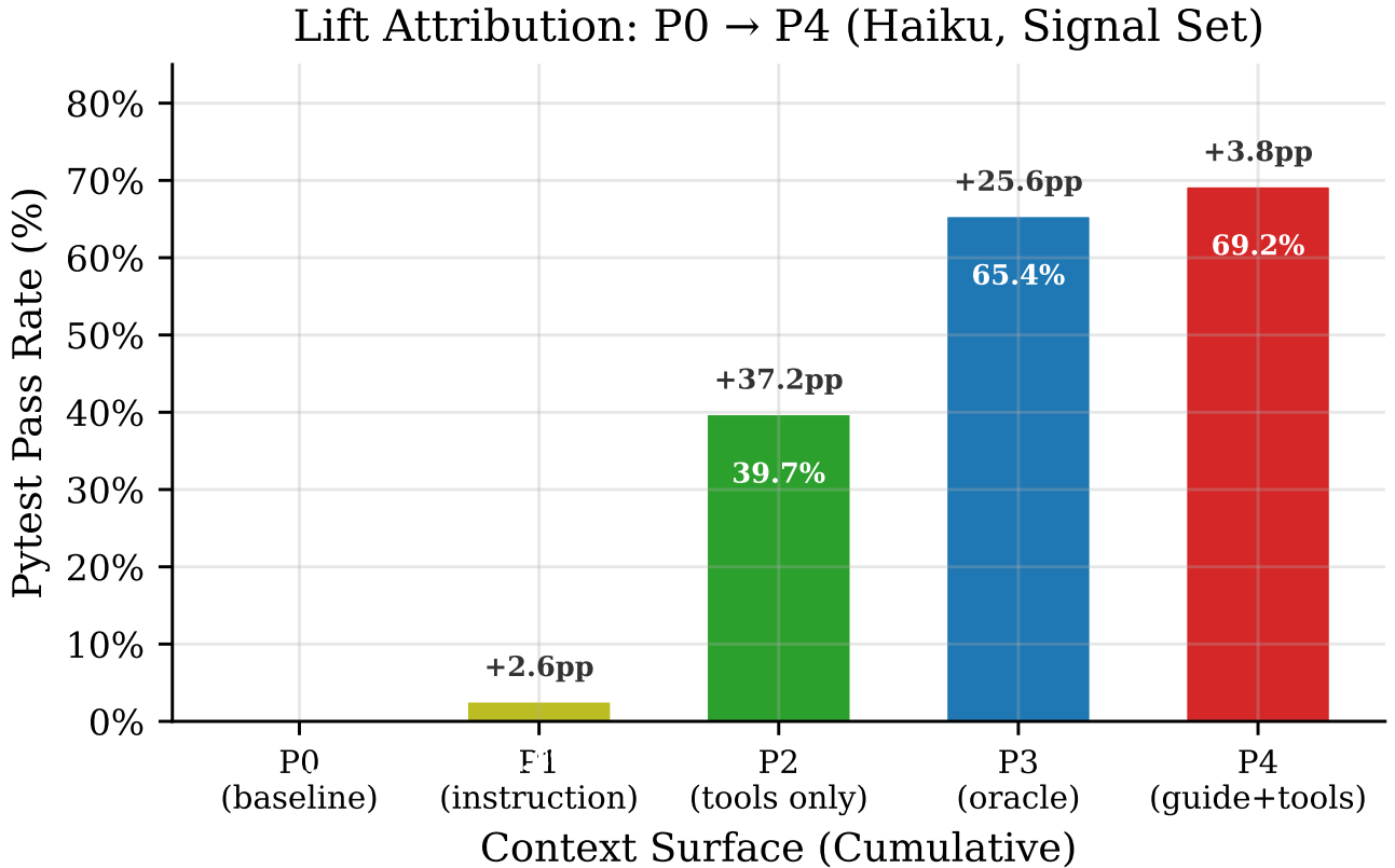
Figure 2: Cumulative lift from P0 (baseline) to P4 (highest-scoring variant) for Haiku on the 26-bug signal set. Each bar shows the absolute pass rate; annotations show incremental lift from the previous variant.
