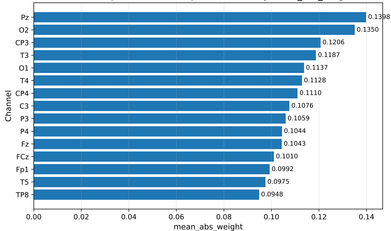
Liu2024 S-JEPA PreLocal - top 15 channels by mean_abs_weight
