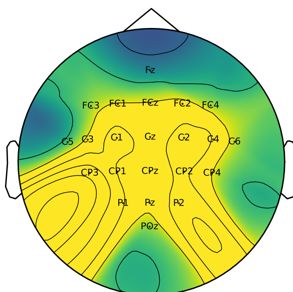
BNCI2014_001 (n=22)
