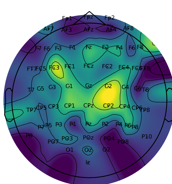
BNCI2014_001 (n=22)
