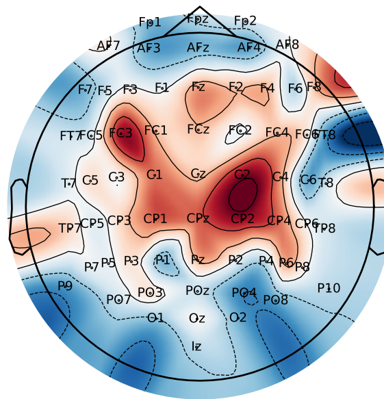
BNCI2014_001 (n=22)
