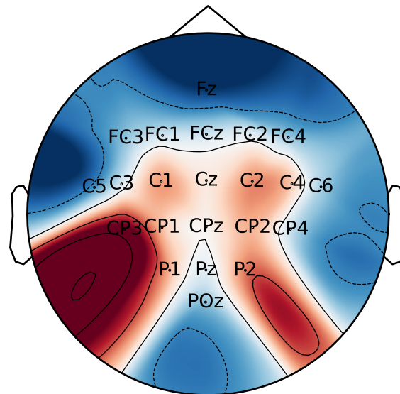
BNCI2014_001 (n=22)
