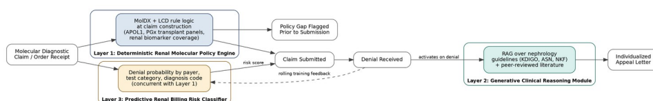
Figure 1. RenalIQ system architecture. Layer 1 applies MolDX/LCD rule logic at claim construction while Layer 3 concurrently scores denial probability; Layer 2 activates only on denial receipt, drawing on a nephrology-specific retrieval-augmented knowledge base.
