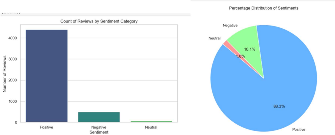
Fig 1: Sentiment Counts
