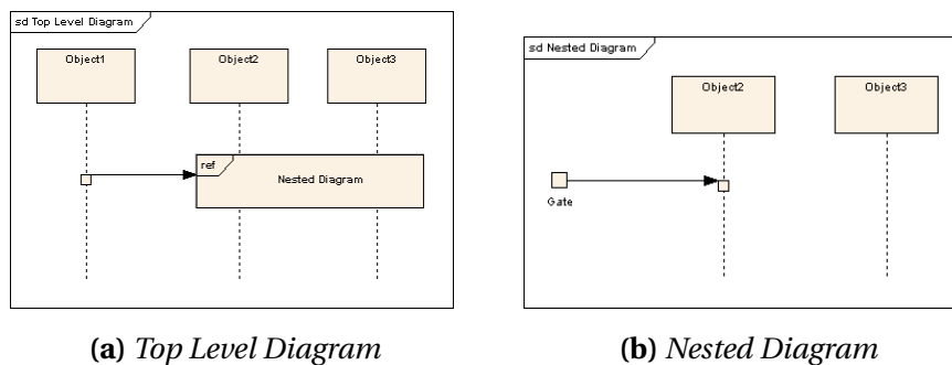
Figure 3.7: Nested Sequence Diagrams
