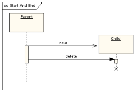
Figure 3.4: Object-Lifetime Start and End
