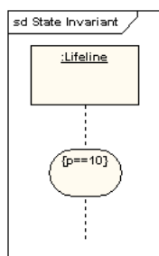
Figure 3.9: State Invariant
