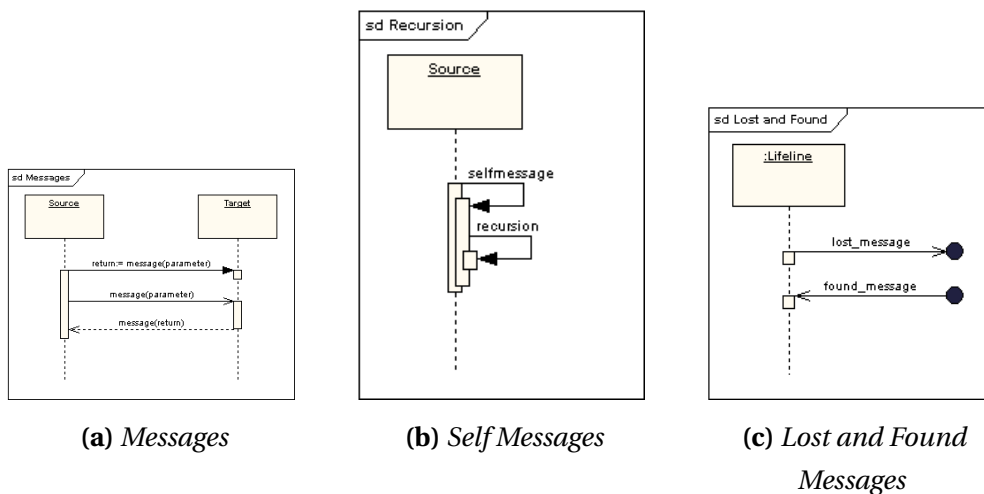
Figure 3.3: Sequence Diagram Messages
