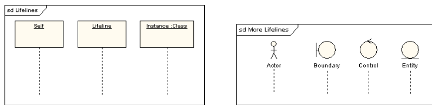
Figure 3.2: Sequence Diagram Lifelines and Actors
