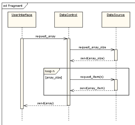
Figure 20.8: Loop Fragment
