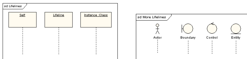
Figure 19.2: Sequence Diagram Lifelines and Actors
