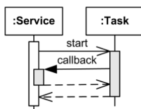
Figure 3.3: Overlapping Execution
