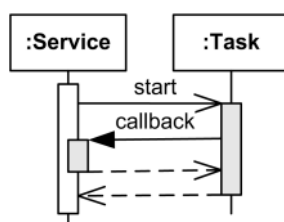
Figure 19.3: Overlapping Execution
