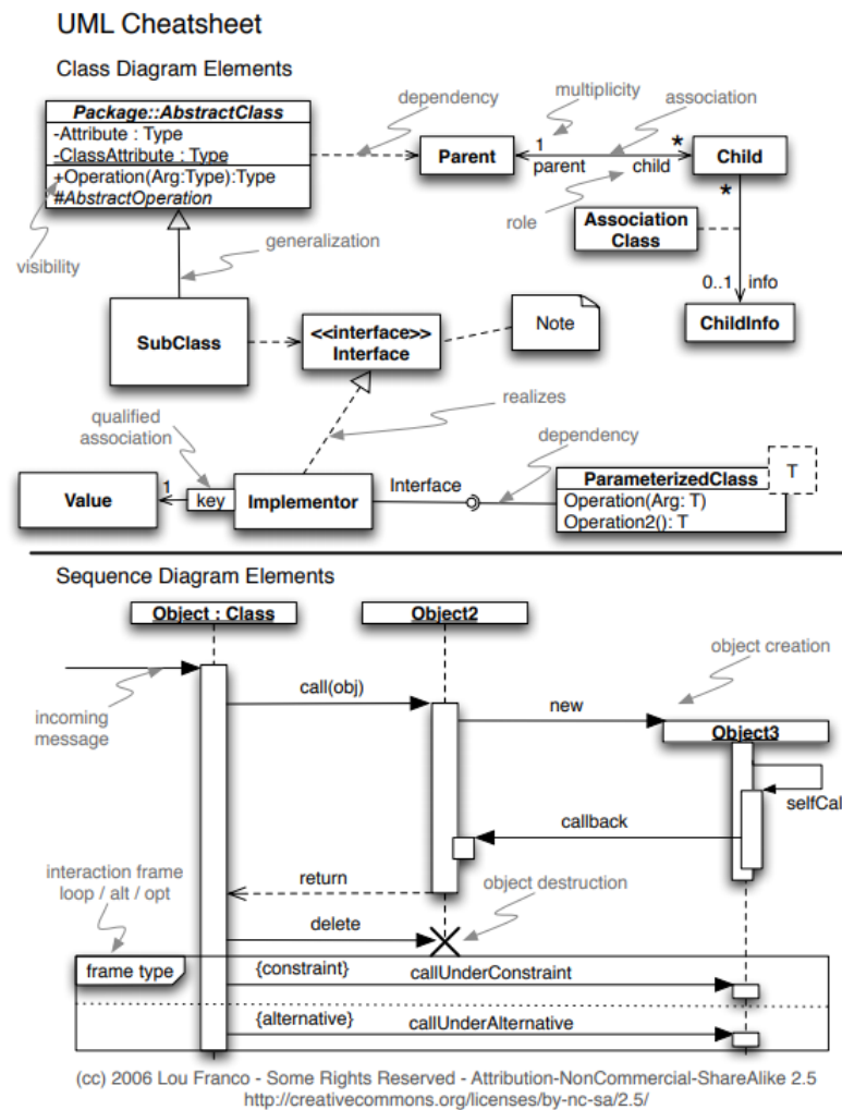
Figure 10.12: Class and Sequence diagrams cheatsheet
